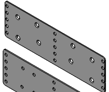
Shoe Plate 0332 (Anka Type)
