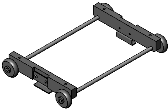
Single Action (Nylon) Carriage 0015K
