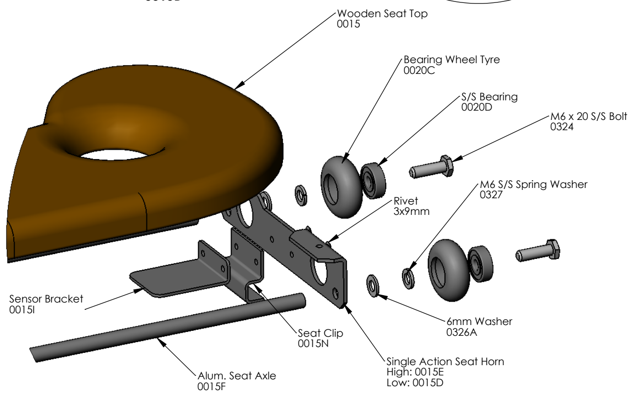
Single Action Bearing Seat 0015B
